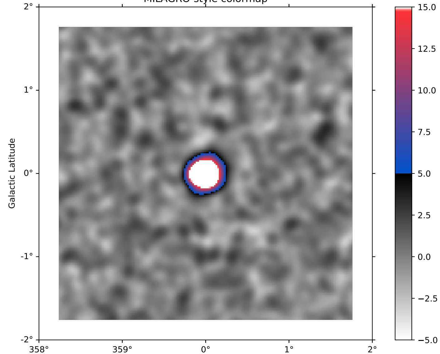
MILAGRO-style colormap
