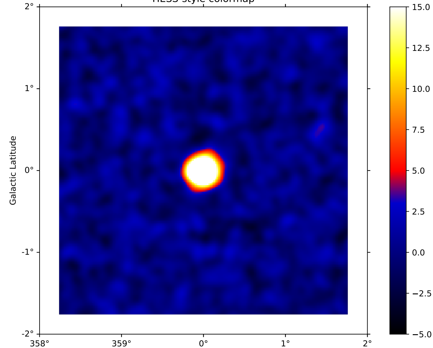
HESS-style colormap
